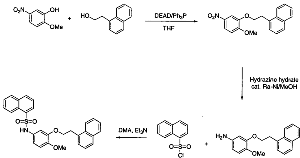
Scheme XII
